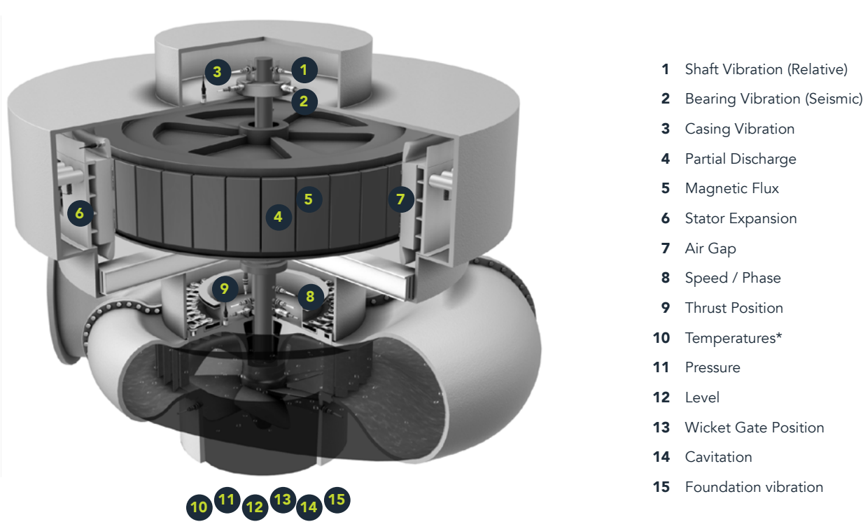
Figure 3: Hydro turbine-generator machines have a number of conventional as well as specialized measurement requirements. Even on conventional measurements, such as radial vibration, requirements are different than on other machine types such as the need to address very low frequencies (down to 0.1 Hz) and the ability to provide signal conditioning such as NOT 1X that can detect the presence of rough load zone.
