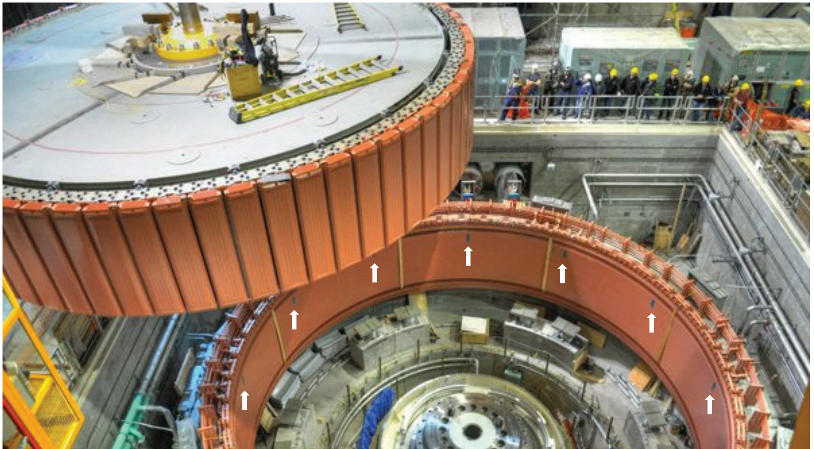
Figure 2: A hydro generator rotor being lowered into place. Note the relative size of the ladder atop the rotor and of the workers along the railings. Such massive sizes are quite common in many hydro plants where vertically oriented turbine-generator units are used. Note also the single layer of stator-mounted air gap sensors (seven are visible) as indicated by the white arrows.
