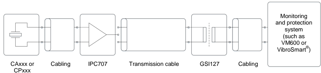
IPC707 output signal
